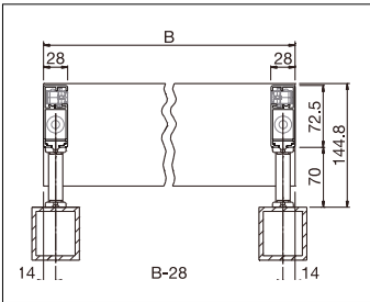
B = Ancho total
