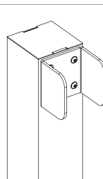
Entronque interior estructura 100x100
