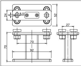
PS401/2 Soporte
