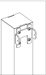
Entronque interior guía 100x120
