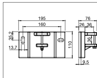
S221/3 Soportes pared
